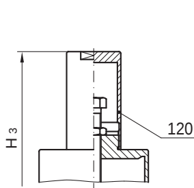
Valve with top cap (Option AC)
