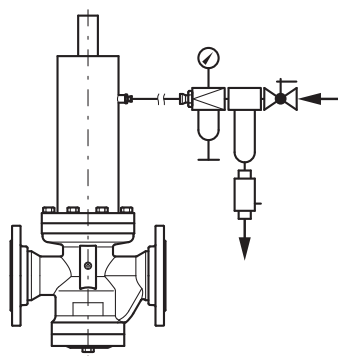
selected reduced pressure by air loading design of the bonnet. (Option EA)
