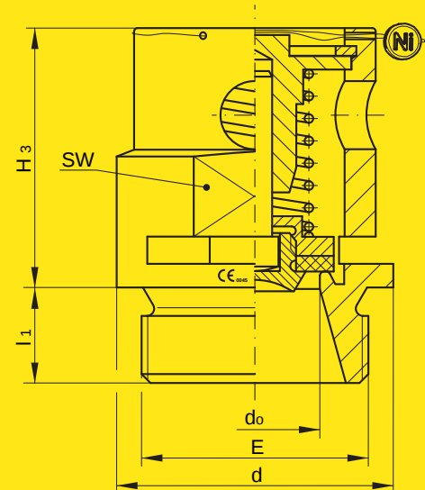
Kopf D, Lüfteknopf head D, lifting button Sonder-Anlüftung special-lifting
