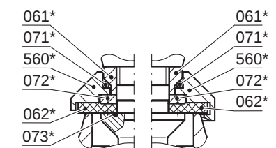
disc complete, pos. 060* Thermoplast seated Elastomer seated
